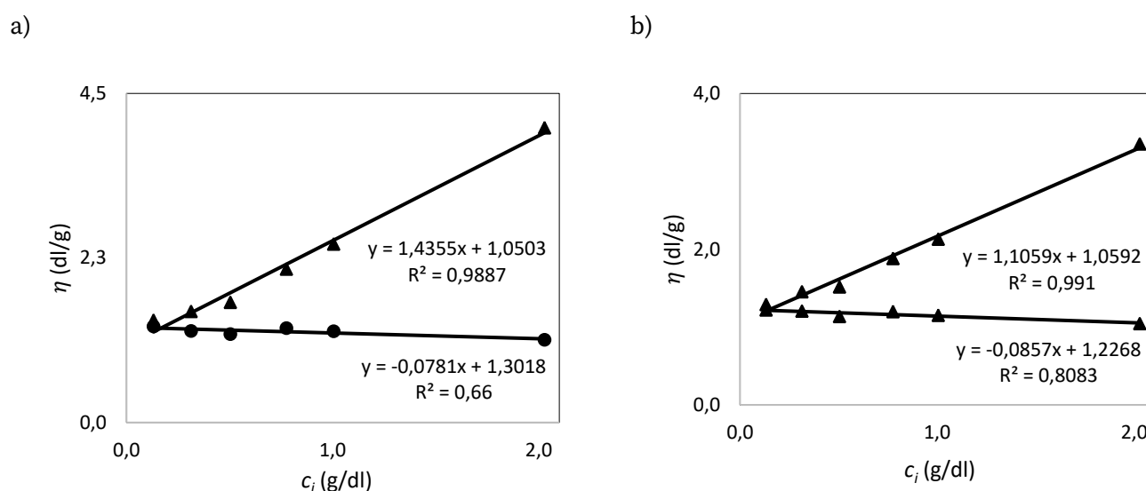
Figura 2. PLA 2003D: \eta_{red} ( \blacktriangle ) y \eta_{inh} ( \bullet ) a 25 °C (a), y 30 °C (b).
